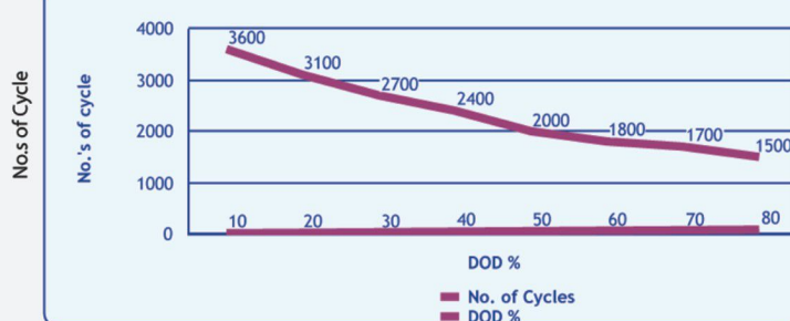
Graph 2: Cycle Life Vs DOD
