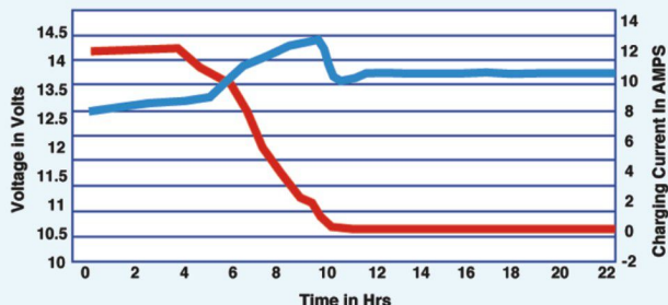
Charging Characteristics
